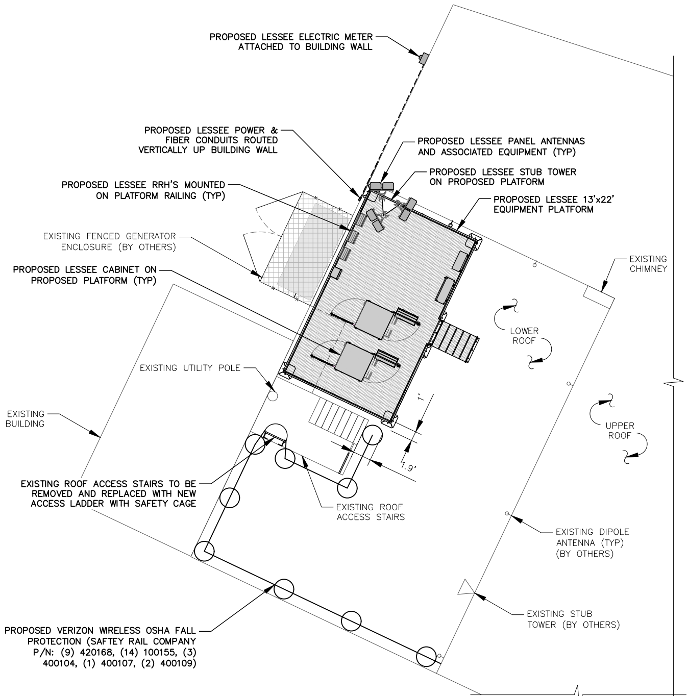
1 ROOF PLAN LE-2 SCALE: 1" = 10'
